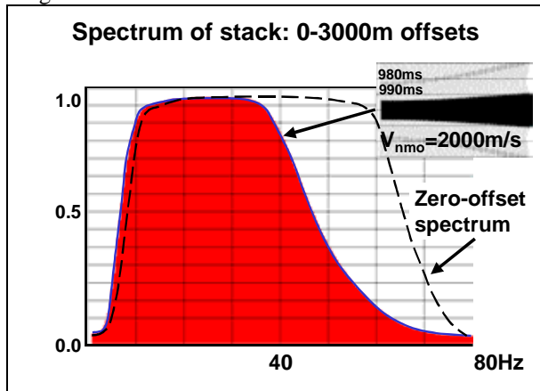
Figure 14: Both frequency content and amplitude are lost due to mis-stacking.
