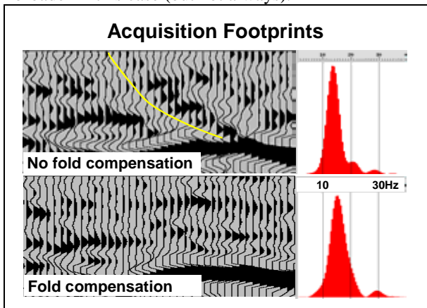
Figure 18: Impulse response noise for data not pre-conditioned to compensate for surface sampling irregularity. The spectrum of the compensated data is broader in this case (but not always).
