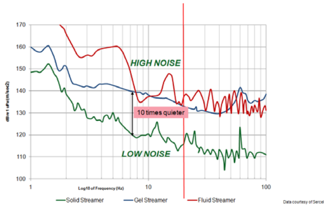
Figure 4: Steamer Vibration Sensitivity Curves (data courtesy of Sercel)
