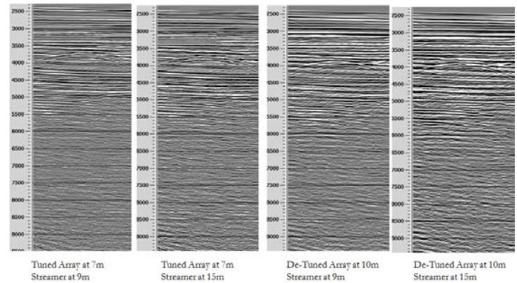
Figure 8: Brute stack with 20 Hz low-pass filter applied
