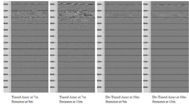
Figure 7: Brute stack sections with 40 Hz high-pass filter applied
