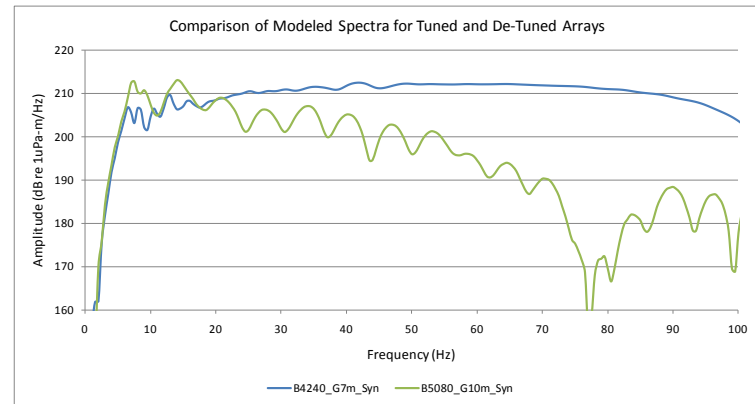
Figure 3: Comparison between tuned array and de-tuned array amplitude spectra
